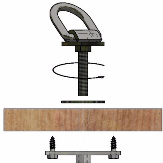
DR1S cutaway
